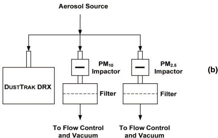
Figure 36: Experimental Setup for (a) Serial and (b) Parallel Gravimetric Calibration
