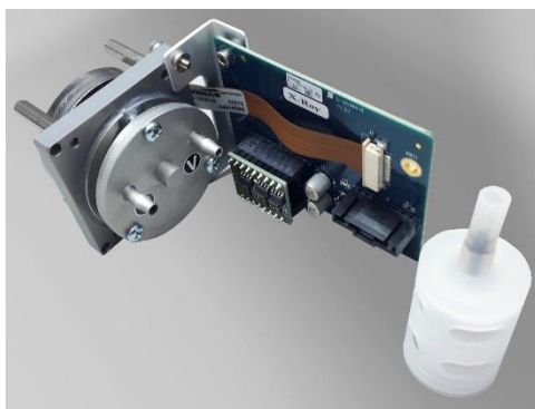
Figure 24: Replacement pump (854043)
