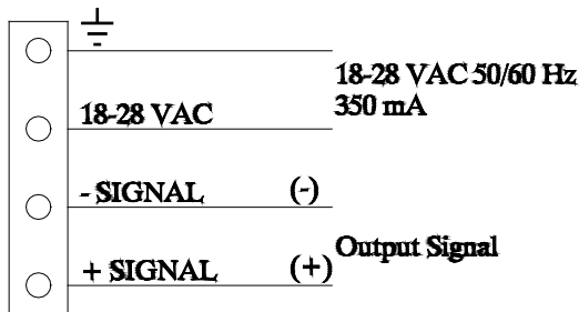
Wiring for AC-Powered Operation
