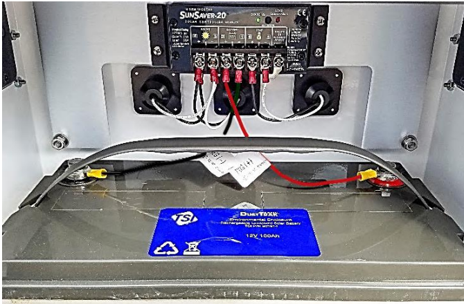
Figure 27: Install the Solar Battery and Connect to Controller
