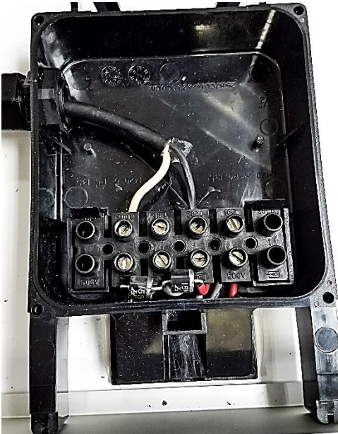
Figure 31: Secure Terminal Block and Tighten Strain Relief
